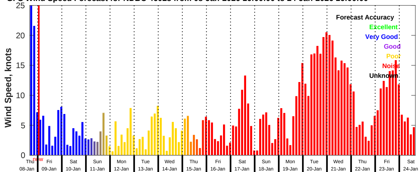
GFS Wind Speed Forecast for NDBC 46028 from 08-Jan-2026 16:00:00 to 24-Jan-2026 16:00:00
