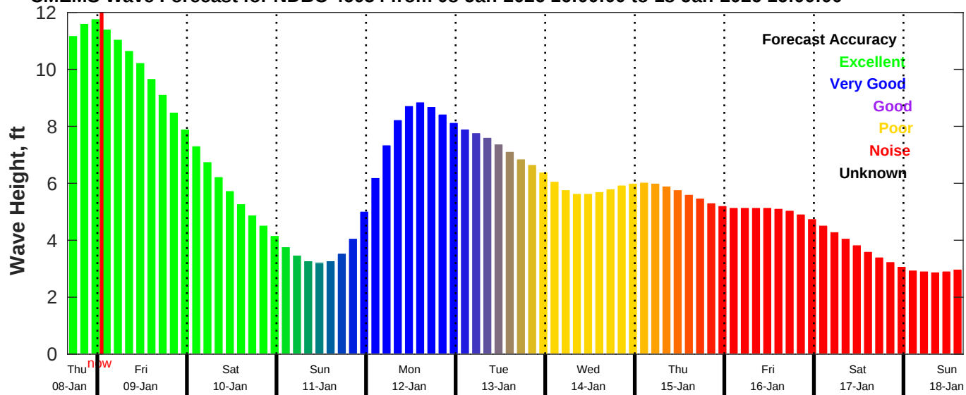
CMEMS Wave Forecast for NDBC 46054 from 08-Jan-2026 16:00:00 to 18-Jan-2026 16:00:00
