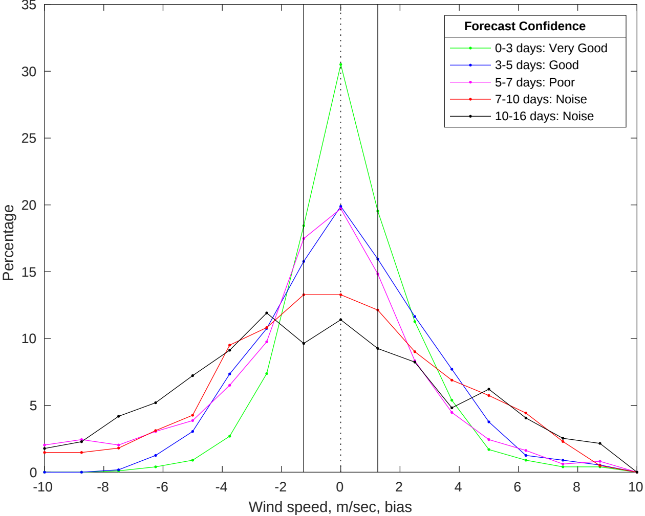
NDBC 46059 vs GFS Winds Bias Histogram: 09-Jan-2026
