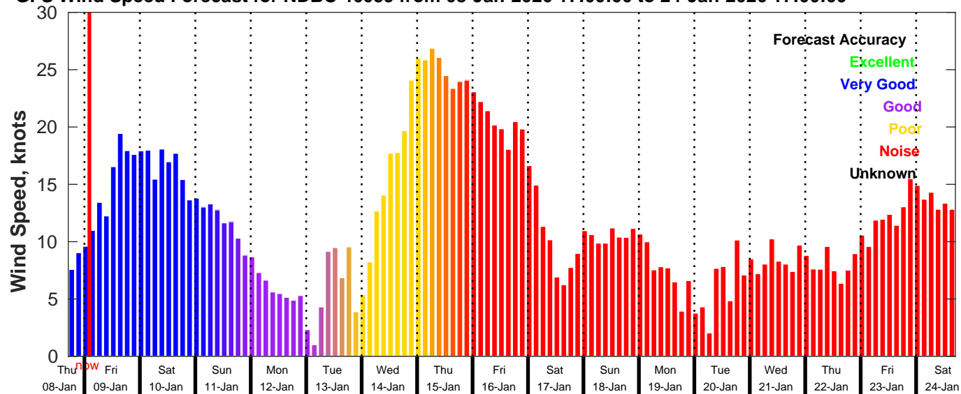
GFS Wind Speed Forecast for NDBC 46059 from 08-Jan-2026 17:00:00 to 24-Jan-2026 17:00:00
