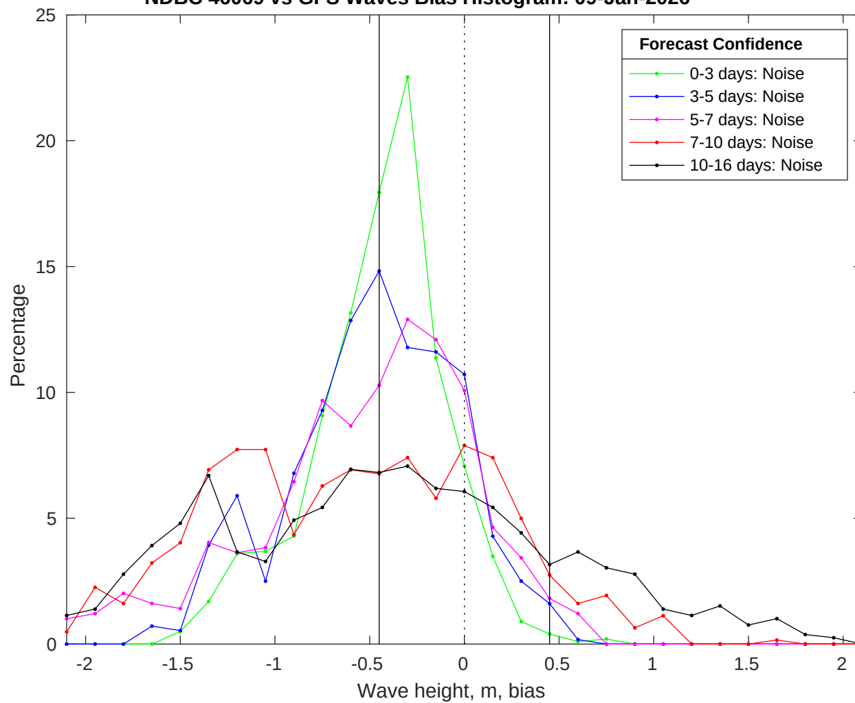
NDBC 46069 vs GFS Waves Bias Histogram: 09-Jan-2026
