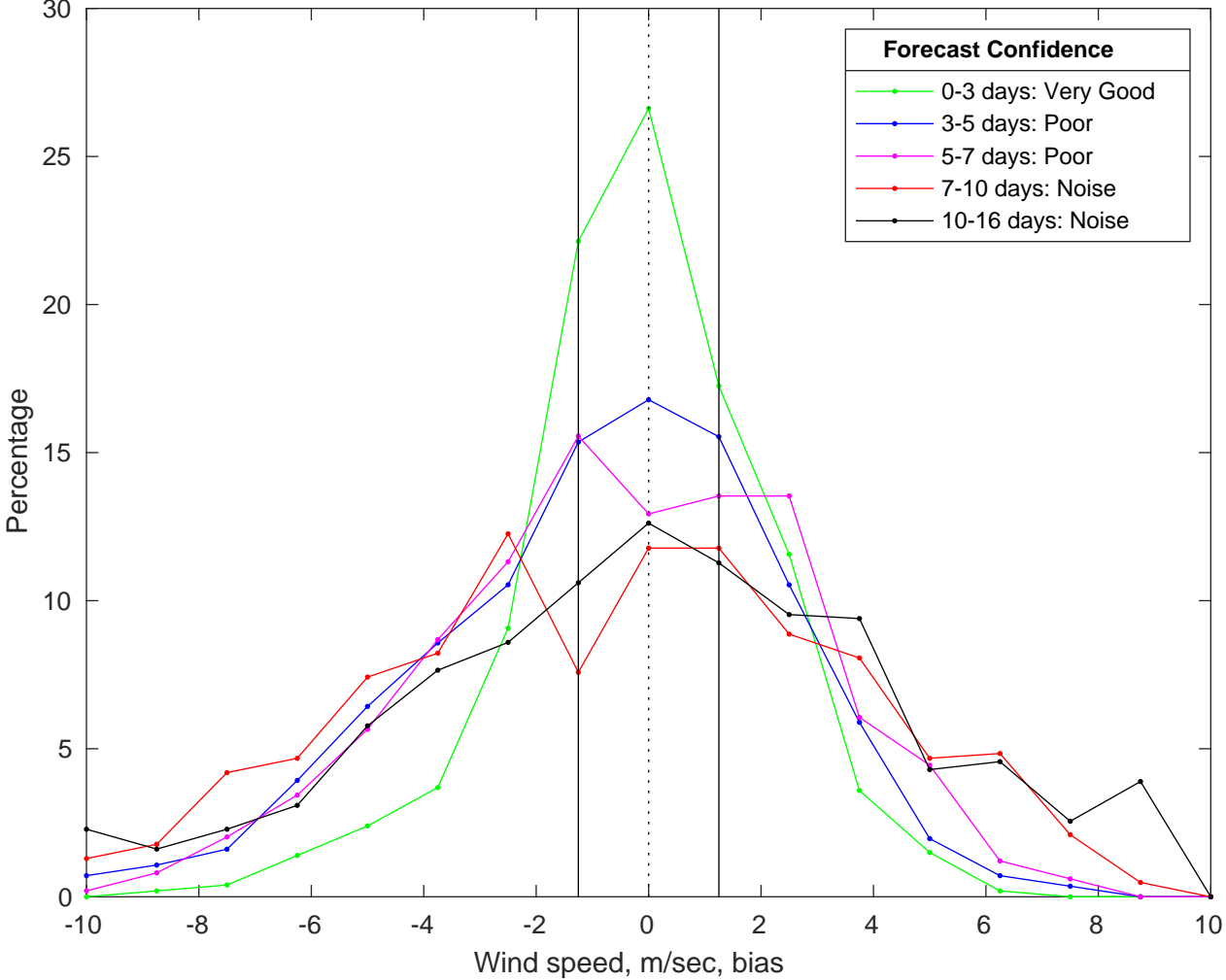
NDBC 46069 vs GFS Winds Bias Histogram: 09-Jan-2026
