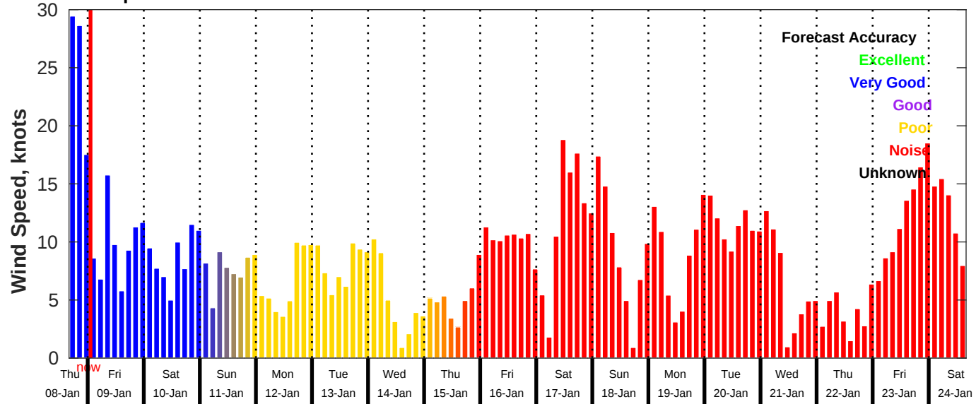
GFS Wind Speed Forecast for NDBC 46069 from 08-Jan-2026 16:00:00 to 24-Jan-2026 16:00:00
