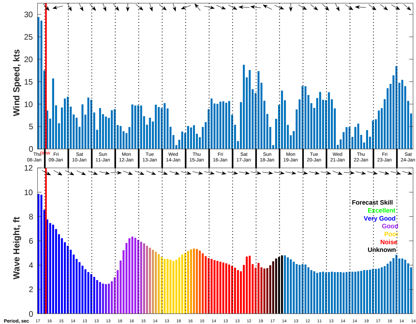
Wind & Wave Forecast for NDBC 46069 from 08-Jan-2026 16:00:00 to 24-Jan-2026 16:00:00
