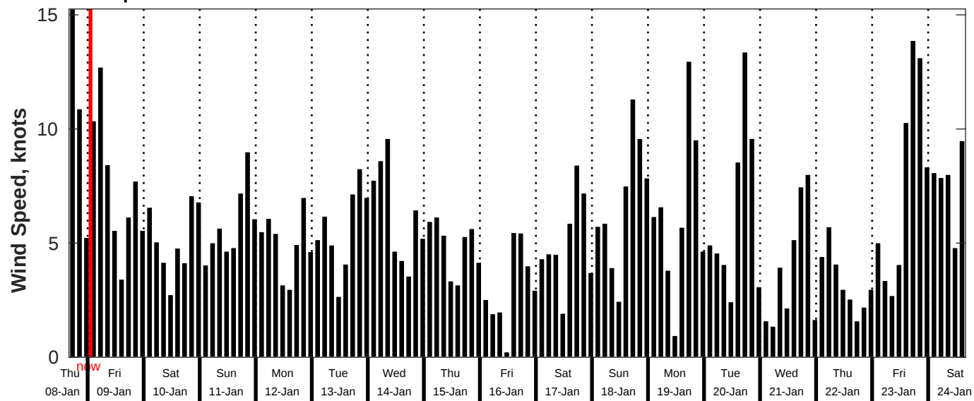
GFS Wind Speed Forecast for NDBC 46215 from 08-Jan-2026 16:00:00 to 24-Jan-2026 16:00:00
