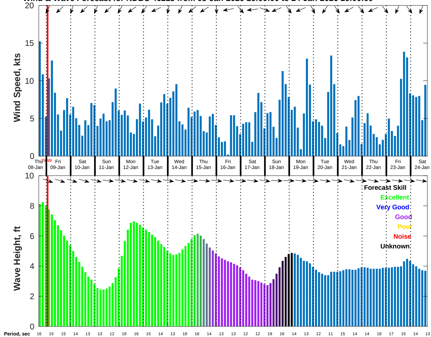
Wind & Wave Forecast for NDBC 46215 from 08-Jan-2026 16:00:00 to 24-Jan-2026 16:00:00
