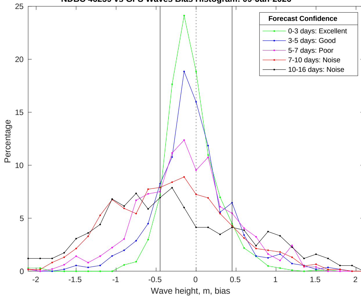
NDBC 46259 vs GFS Waves Bias Histogram: 09-Jan-2026
