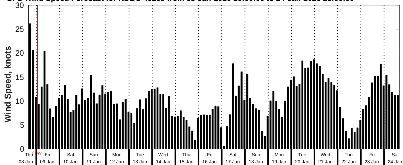
GFS Wind Speed Forecast for NDBC 46259 from 08-Jan-2026 16:00:00 to 24-Jan-2026 16:00:00
