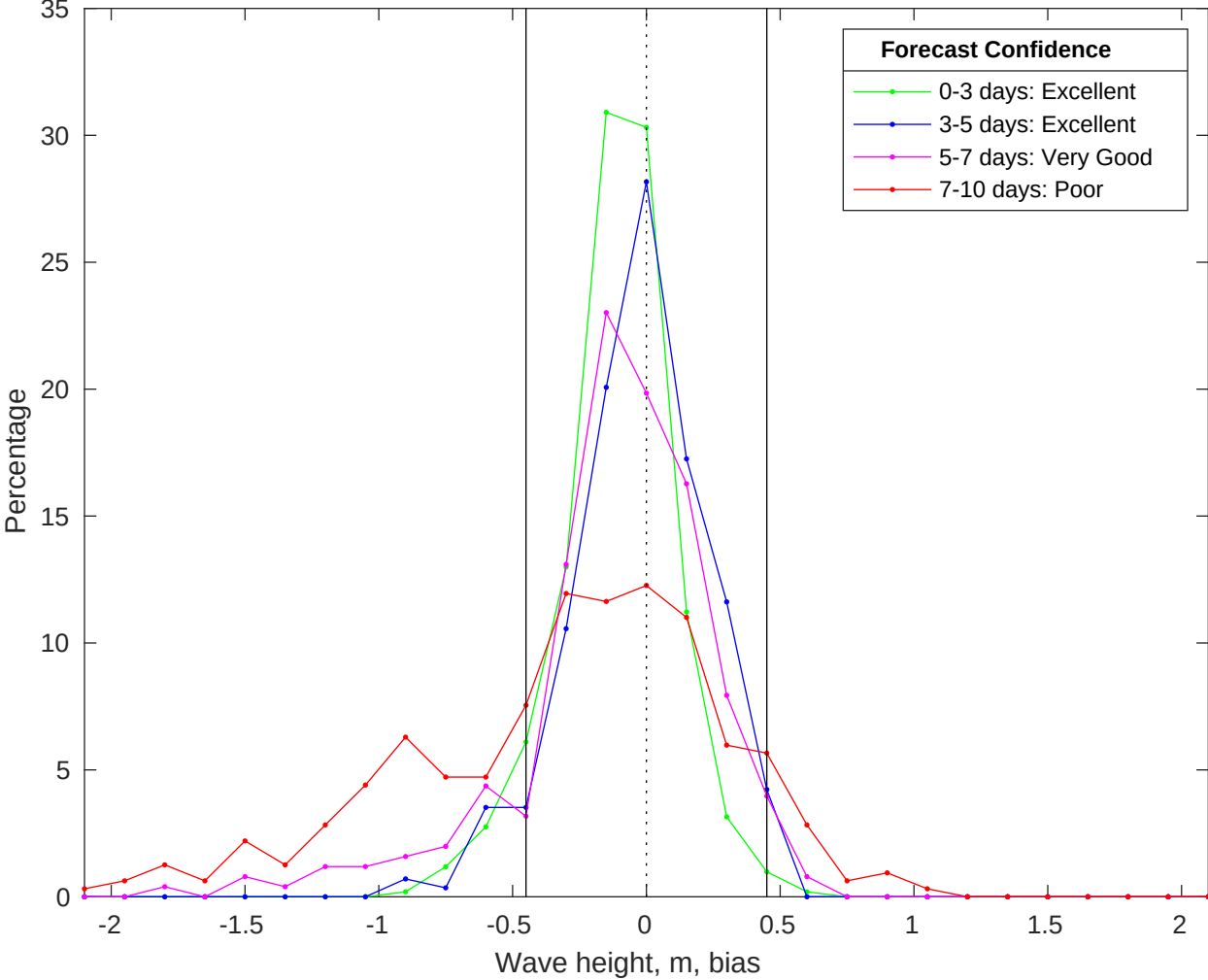
NDBC 51000 vs CMEMS Waves Bias Histogram: 09-Jan-2026
