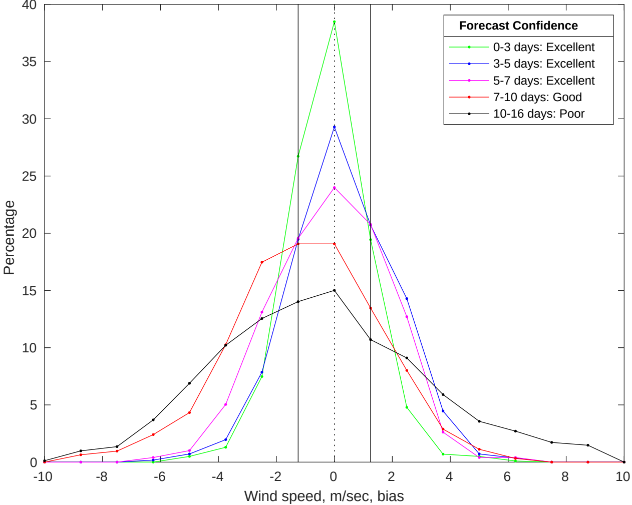
NDBC 51000 vs GFS Winds Bias Histogram: 09-Jan-2026
