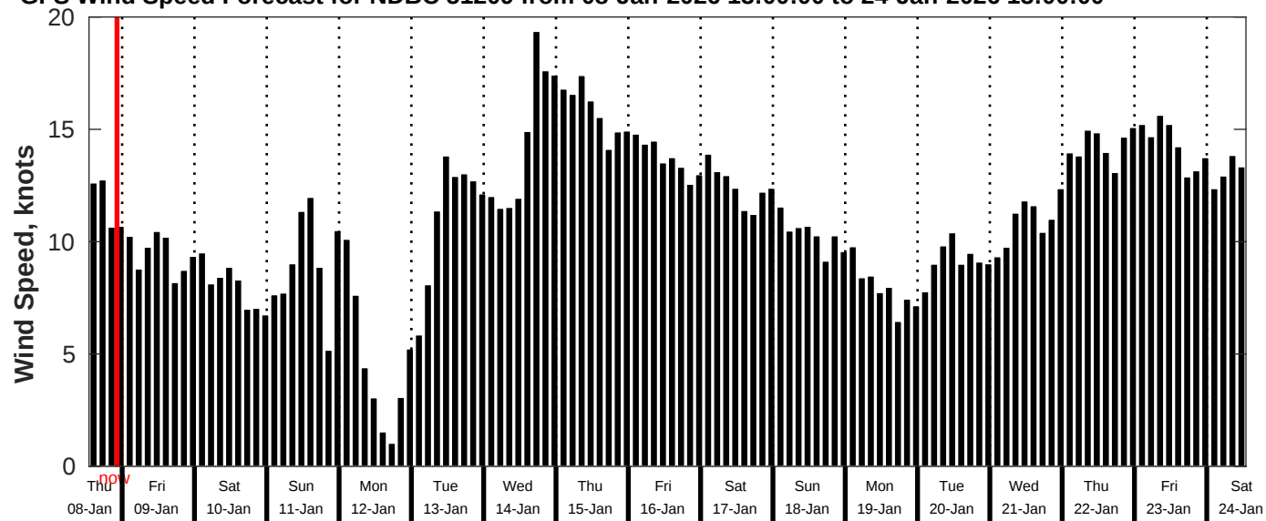
GFS Wind Speed Forecast for NDBC 51209 from 08-Jan-2026 13:00:00 to 24-Jan-2026 13:00:00
