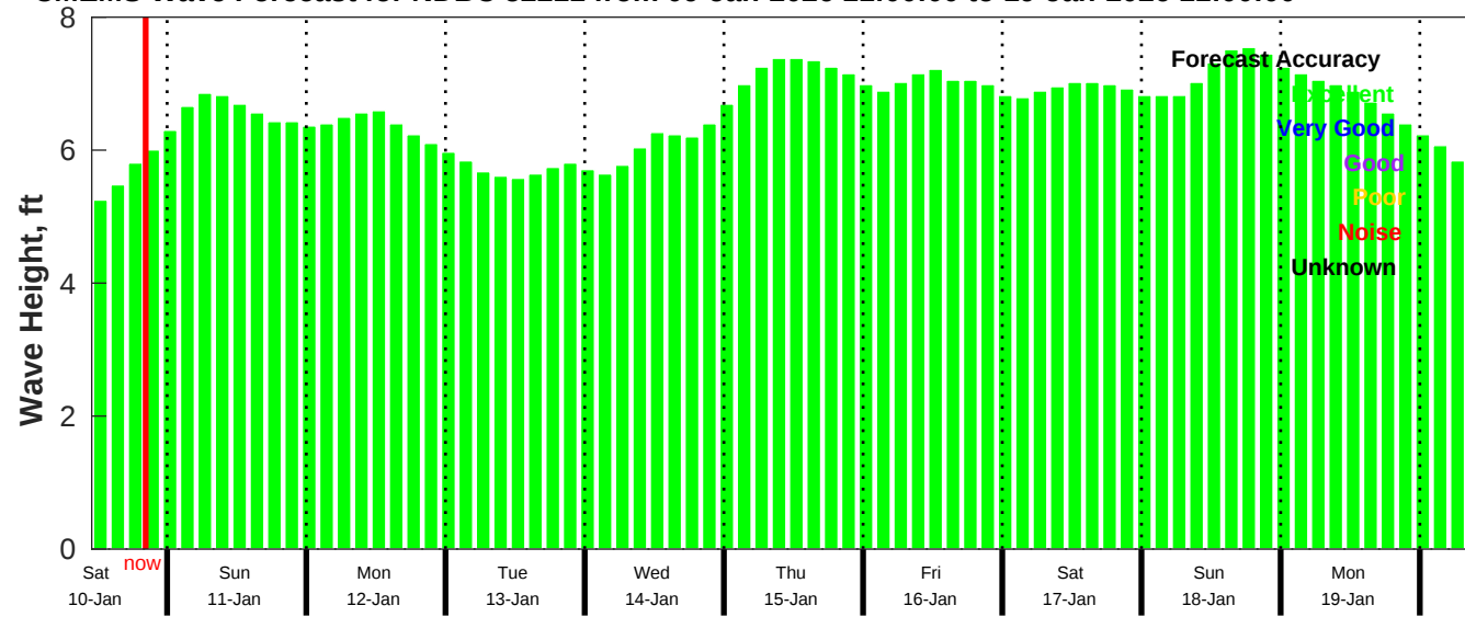
CMEMS Wave Forecast for NDBC 52211 from 09-Jan-2026 11:00:00 to 19-Jan-2026 11:00:00
