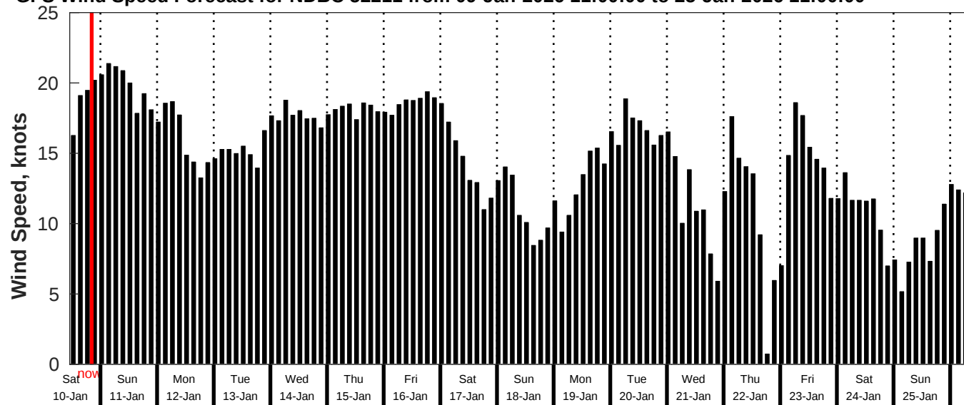
GFS Wind Speed Forecast for NDBC 52211 from 09-Jan-2026 11:00:00 to 25-Jan-2026 11:00:00
