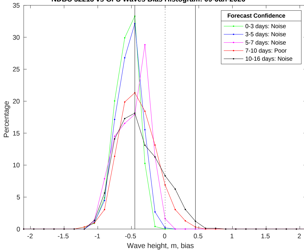
NDBC 52213 vs GFS Waves Bias Histogram: 09-Jan-2026
