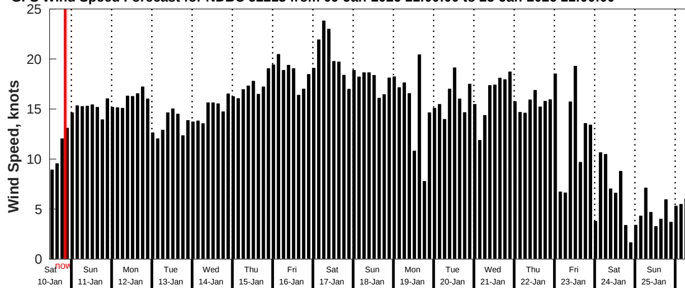
GFS Wind Speed Forecast for NDBC 52213 from 09-Jan-2026 11:00:00 to 25-Jan-2026 11:00:00
