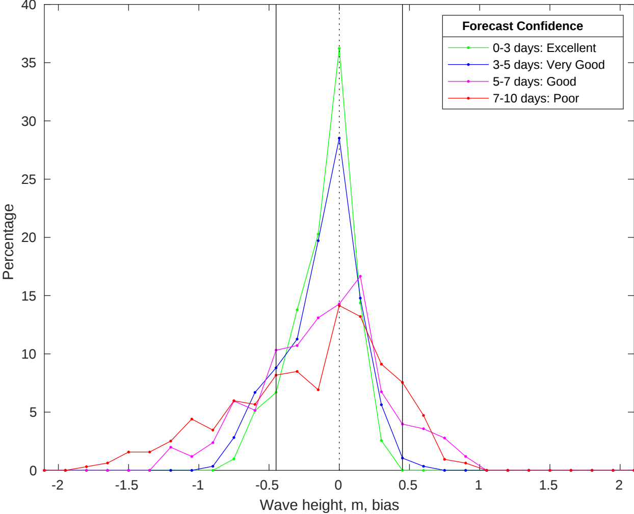
NDBC 41004 vs CMEMS Waves Bias Histogram: 10-Jan-2026
