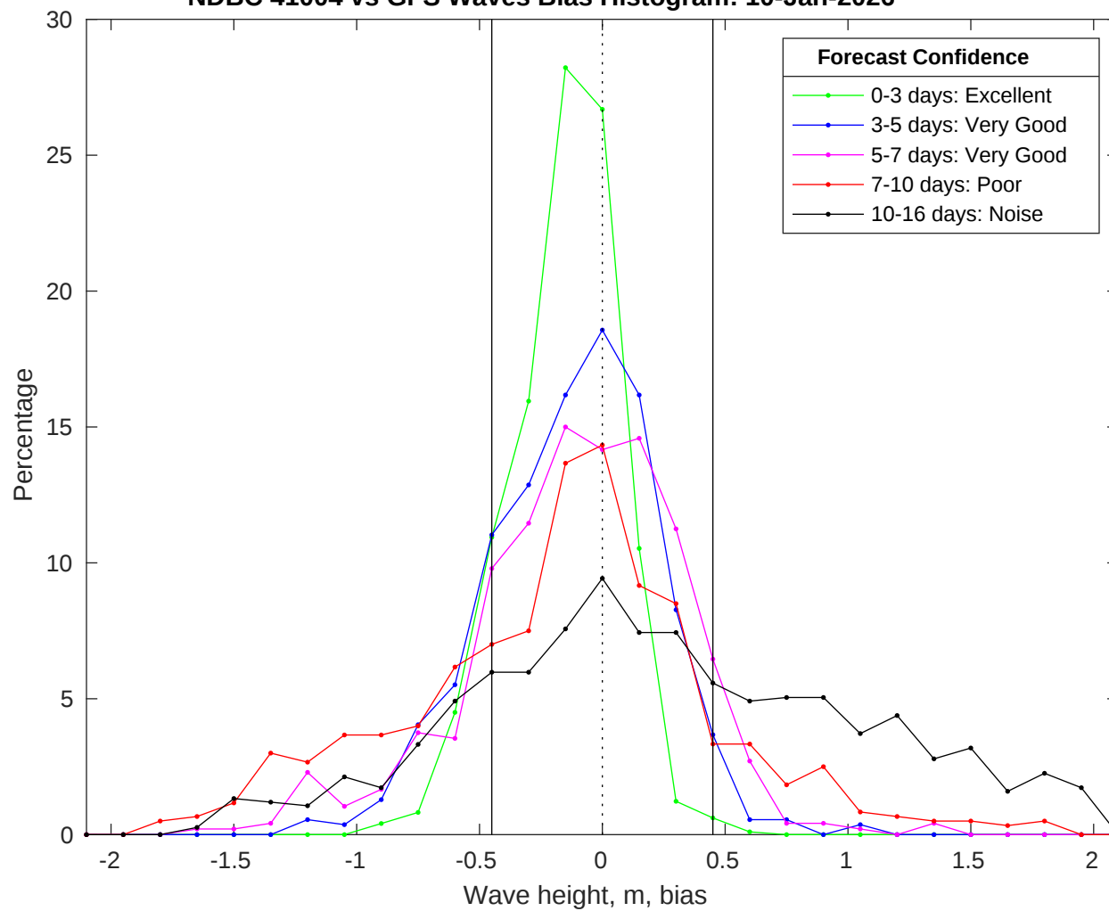
NDBC 41004 vs GFS Waves Bias Histogram: 10-Jan-2026
