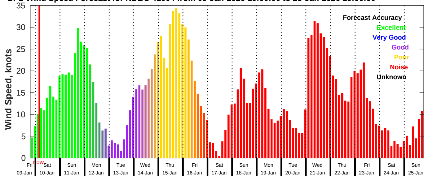
GFS Wind Speed Forecast for NDBC 41004 from 09-Jan-2026 19:00:00 to 25-Jan-2026 19:00:00
