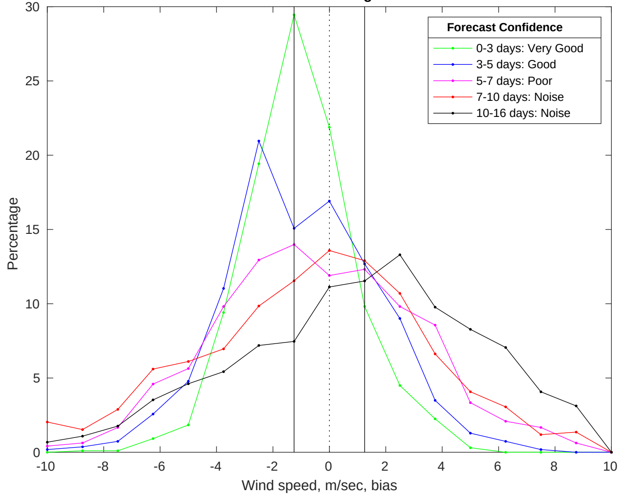
NDBC 41013 vs GFS Winds Bias Histogram: 10-Jan-2026
