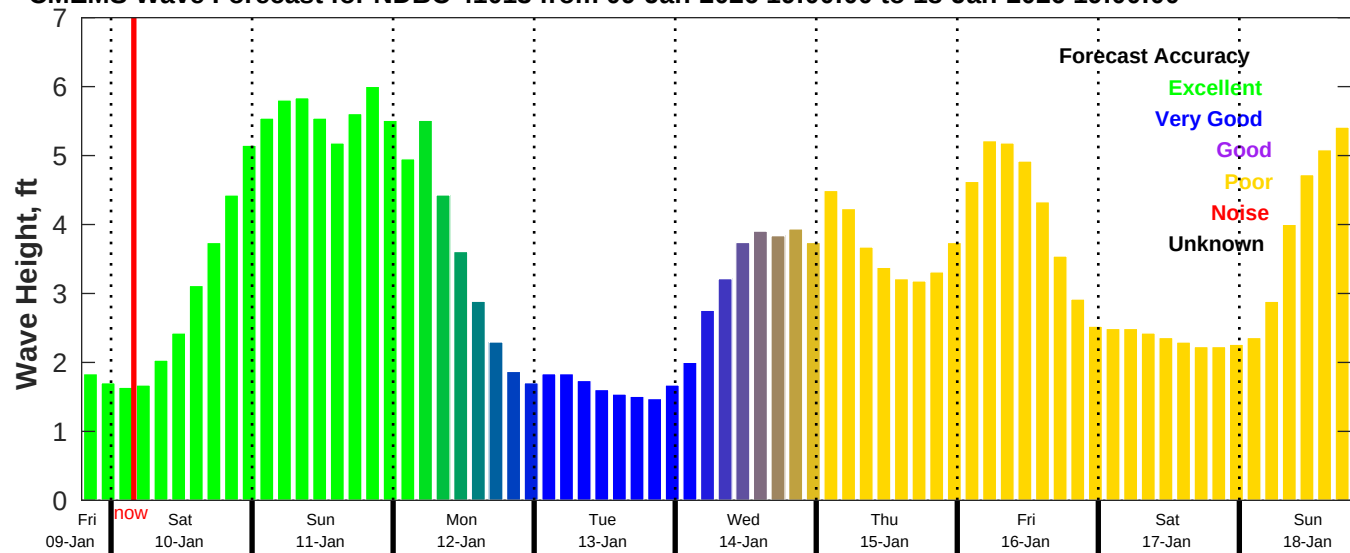
CMEMS Wave Forecast for NDBC 41013 from 09-Jan-2026 19:00:00 to 18-Jan-2026 19:00:00
