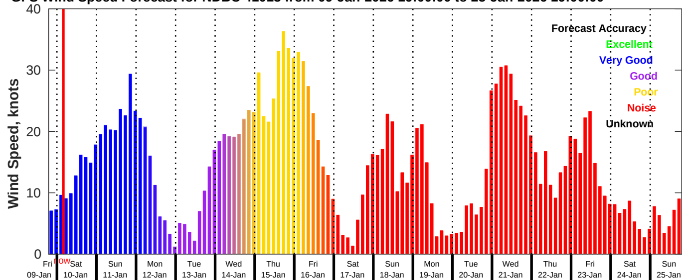
GFS Wind Speed Forecast for NDBC 41013 from 09-Jan-2026 19:00:00 to 25-Jan-2026 19:00:00
