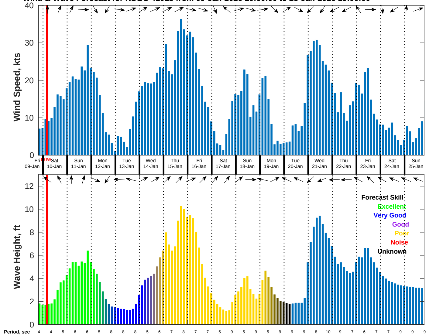
Wind & Wave Forecast for NDBC 41013 from 09-Jan-2026 19:00:00 to 25-Jan-2026 19:00:00
