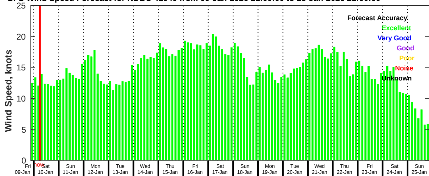
GFS Wind Speed Forecast for NDBC 41040 from 09-Jan-2026 21:00:00 to 25-Jan-2026 21:00:00
