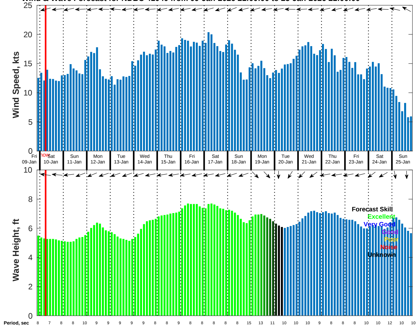
Wind & Wave Forecast for NDBC 41040 from 09-Jan-2026 21:00:00 to 25-Jan-2026 21:00:00
