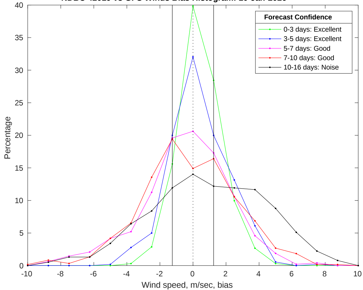
NDBC 42019 vs GFS Winds Bias Histogram: 10-Jan-2026
