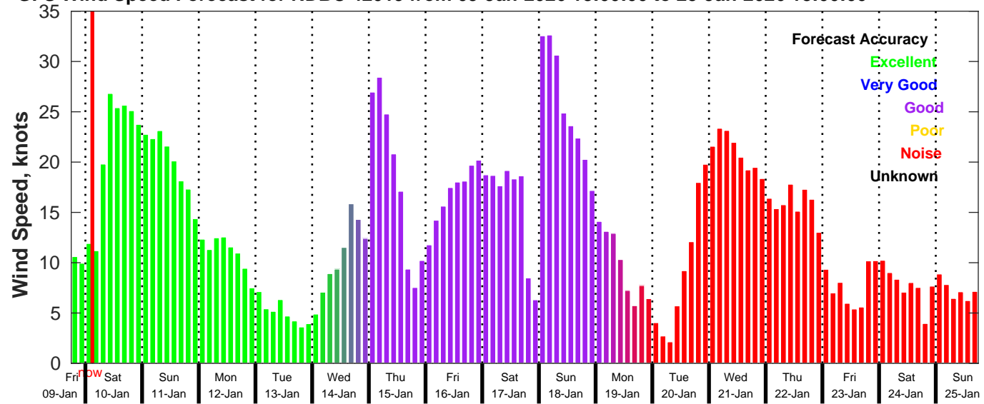
GFS Wind Speed Forecast for NDBC 42019 from 09-Jan-2026 18:00:00 to 25-Jan-2026 18:00:00
