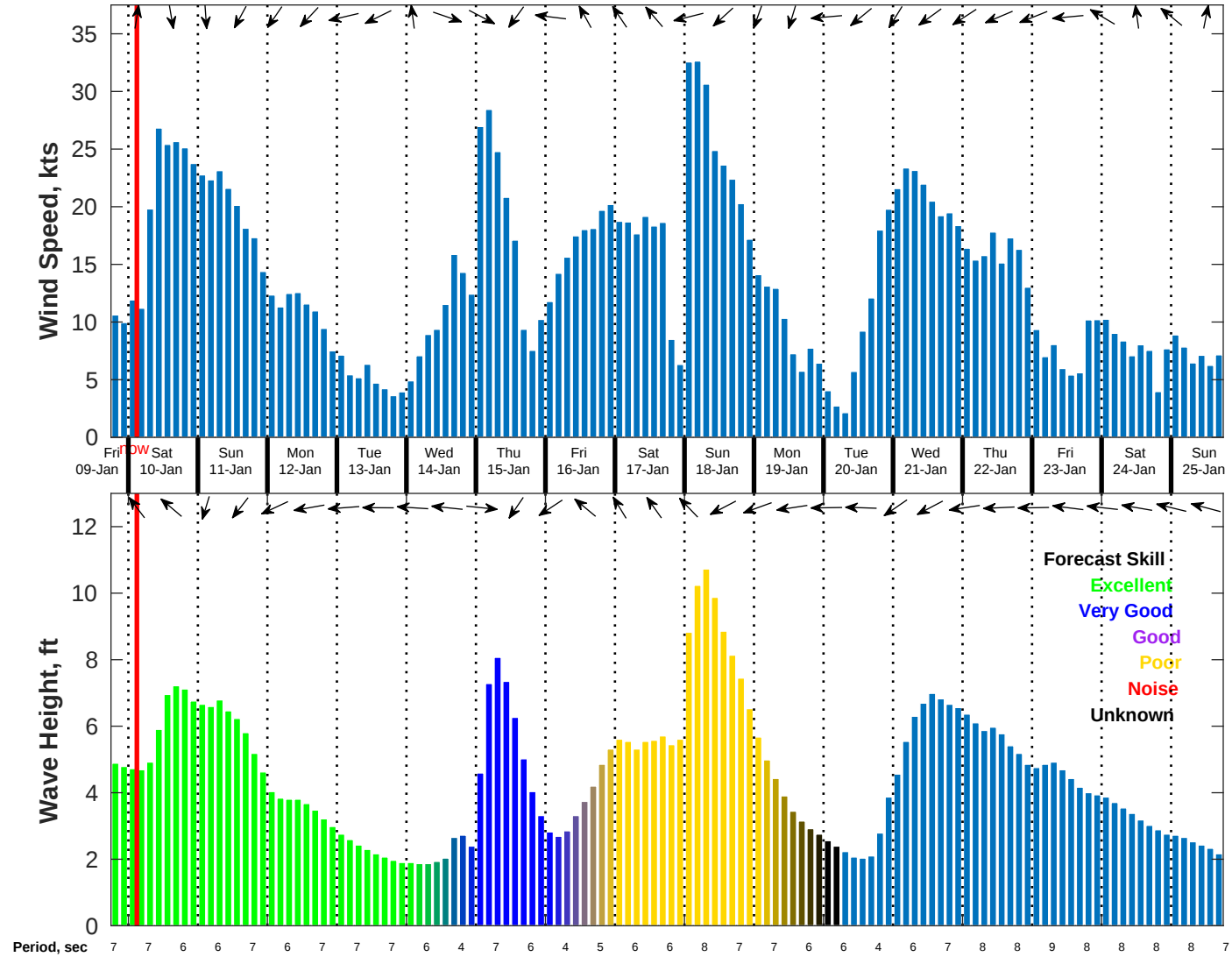
Wind & Wave Forecast for NDBC 42019 from 09-Jan-2026 18:00:00 to 25-Jan-2026 18:00:00
