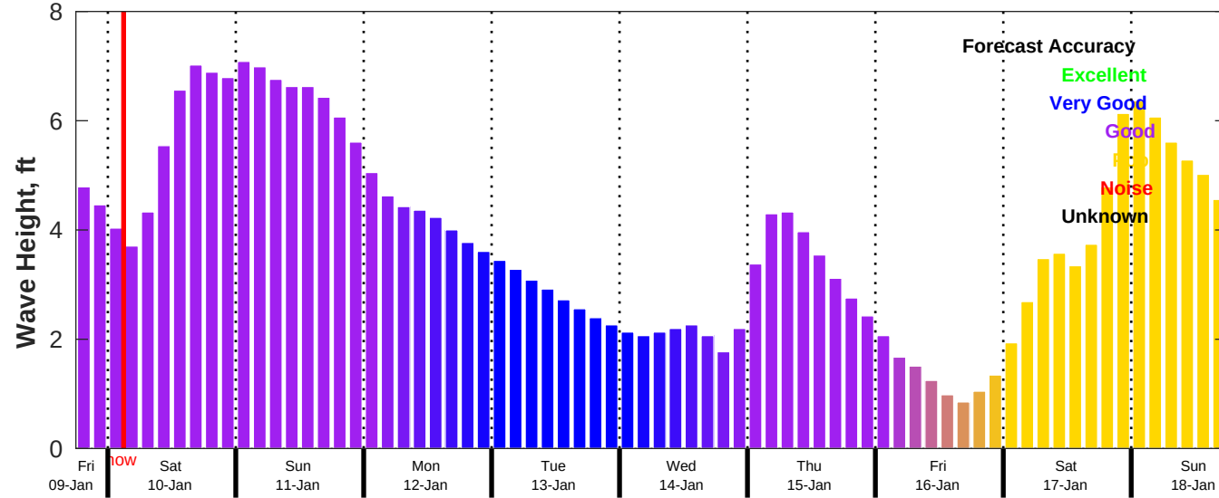
CMEMS Wave Forecast for NDBC 42020 from 09-Jan-2026 18:00:00 to 18-Jan-2026 18:00:00
