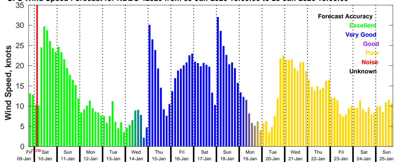
GFS Wind Speed Forecast for NDBC 42020 from 09-Jan-2026 18:00:00 to 25-Jan-2026 18:00:00
