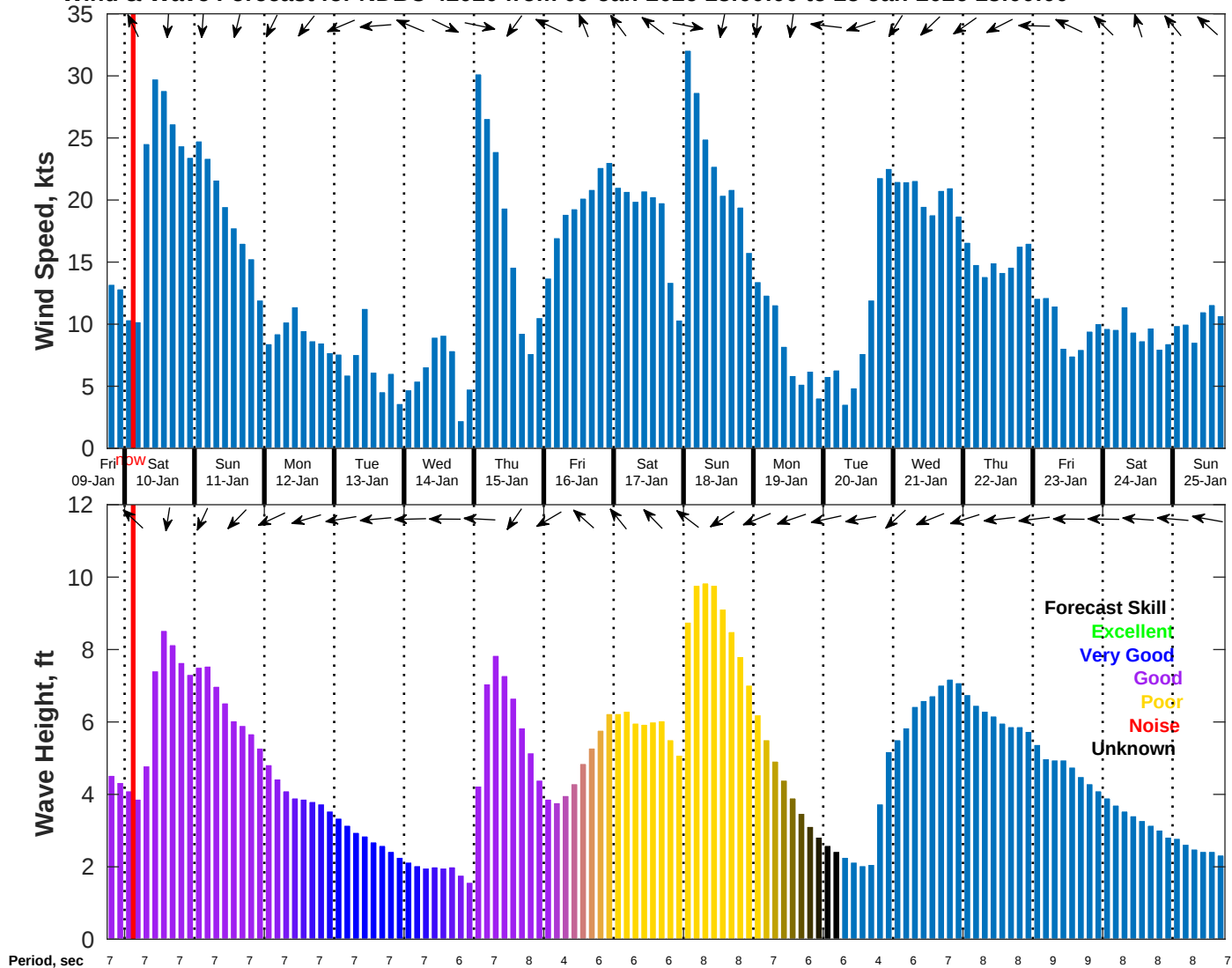
Wind & Wave Forecast for NDBC 42020 from 09-Jan-2026 18:00:00 to 25-Jan-2026 18:00:00
