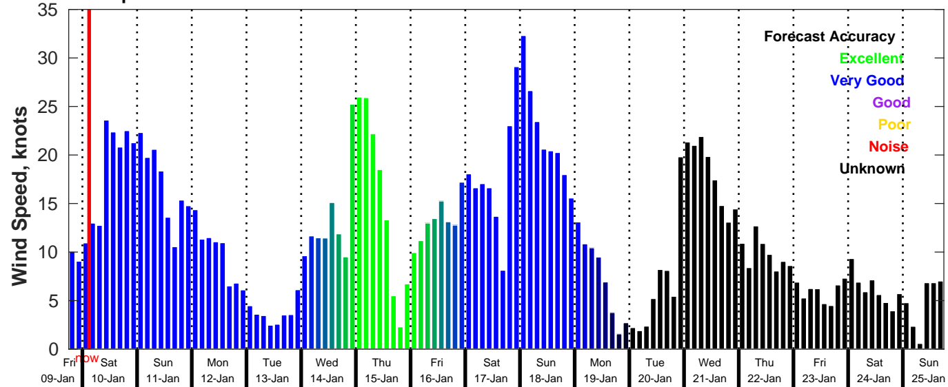
GFS Wind Speed Forecast for NDBC 42035 from 09-Jan-2026 18:00:00 to 25-Jan-2026 18:00:00
