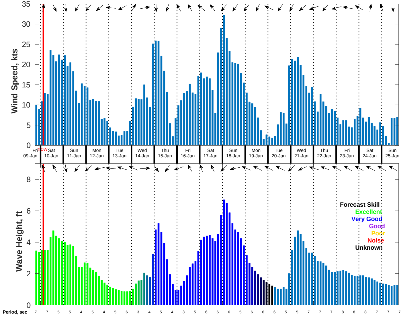
Wind & Wave Forecast for NDBC 42035 from 09-Jan-2026 18:00:00 to 25-Jan-2026 18:00:00
