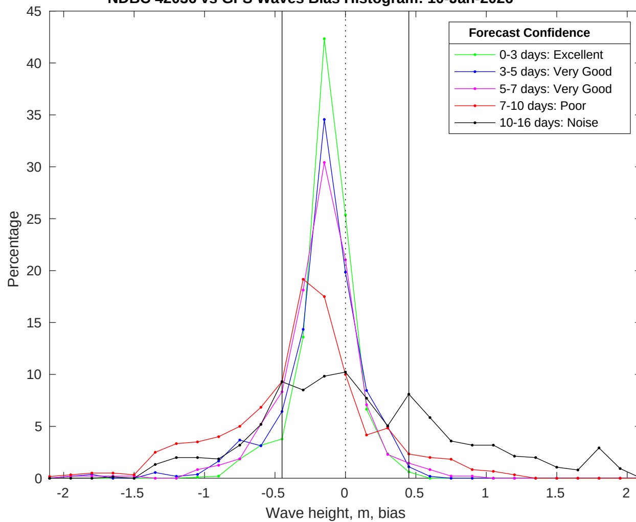
NDBC 42036 vs GFS Waves Bias Histogram: 10-Jan-2026
