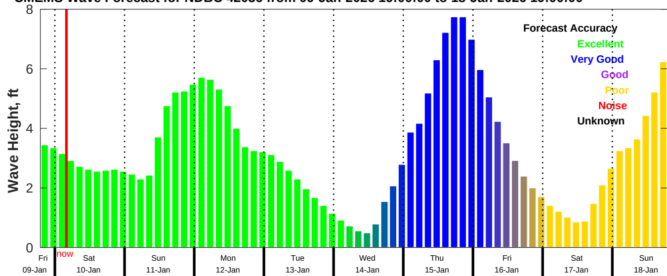
CMEMS Wave Forecast for NDBC 42036 from 09-Jan-2026 19:00:00 to 18-Jan-2026 19:00:00
