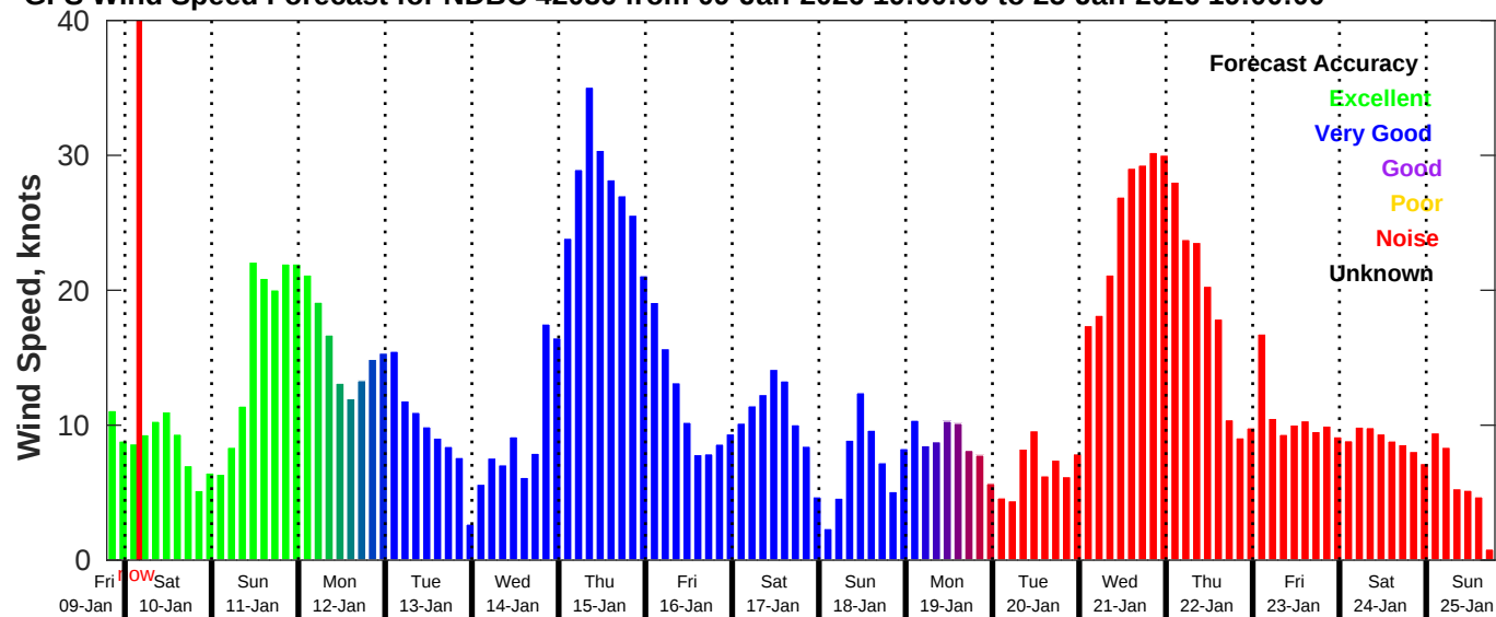
GFS Wind Speed Forecast for NDBC 42036 from 09-Jan-2026 19:00:00 to 25-Jan-2026 19:00:00
