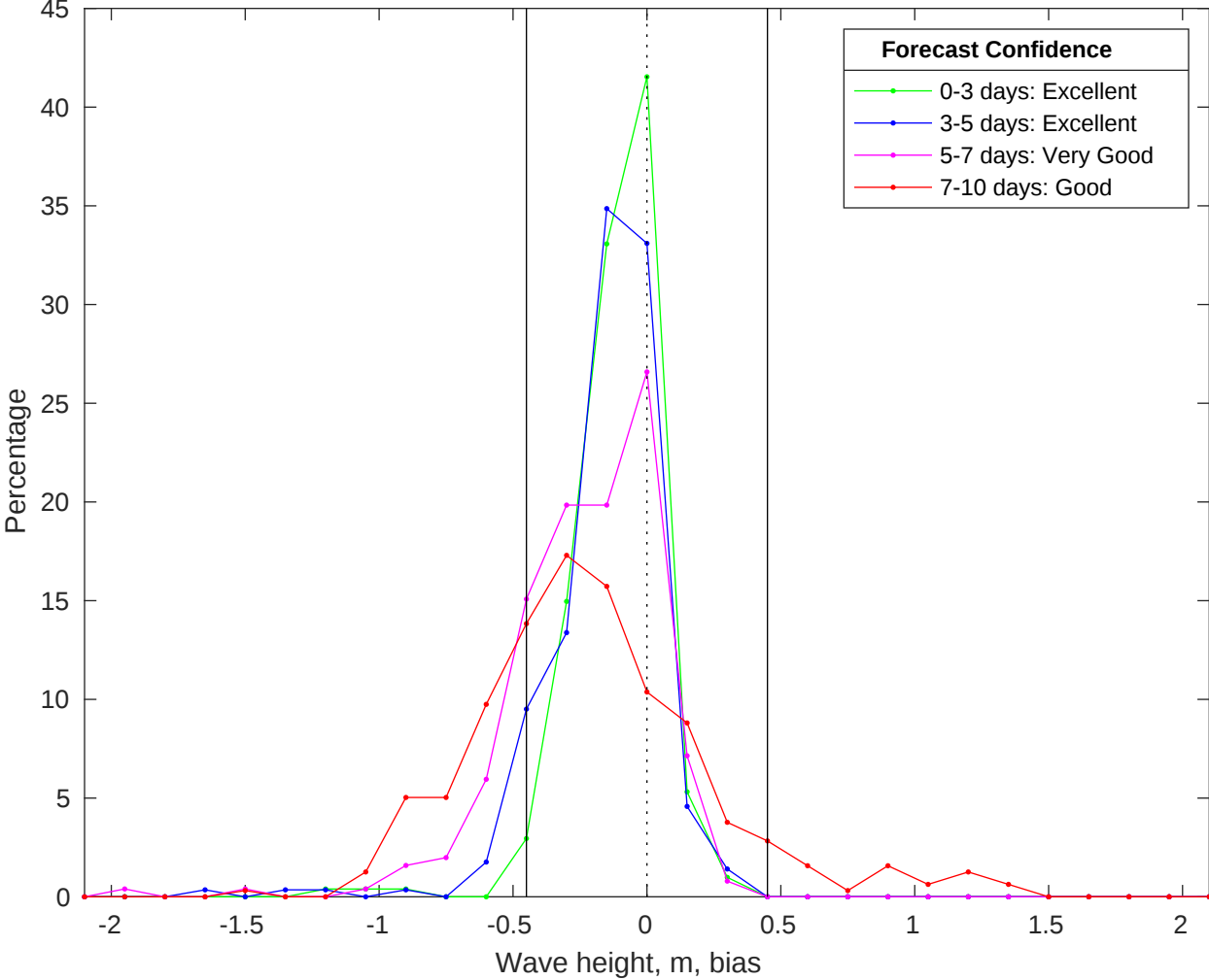
NDBC 42040 vs CMEMS Waves Bias Histogram: 10-Jan-2026
