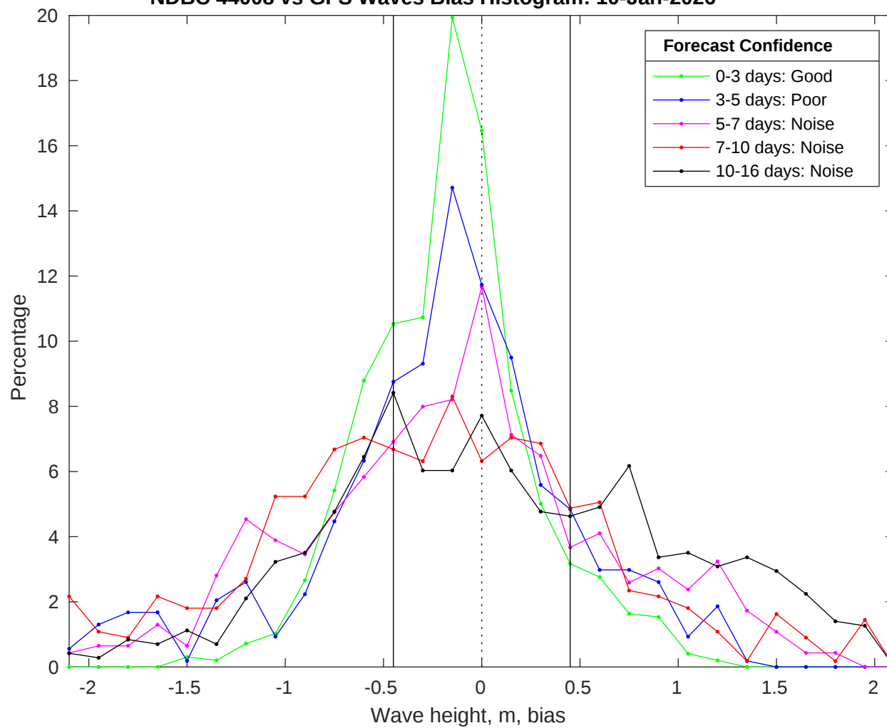
NDBC 44008 vs GFS Waves Bias Histogram: 10-Jan-2026
