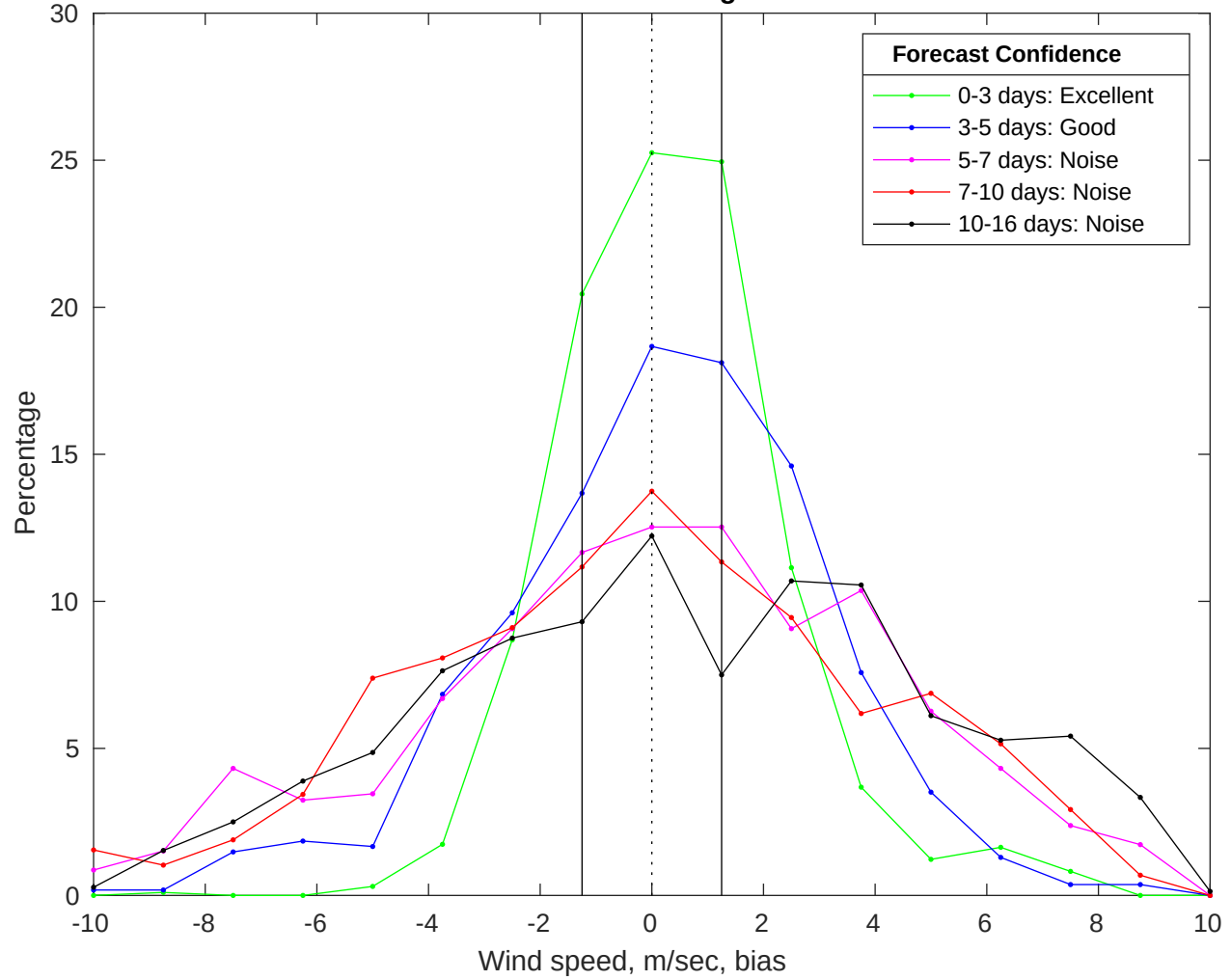
NDBC 44008 vs GFS Winds Bias Histogram: 10-Jan-2026
