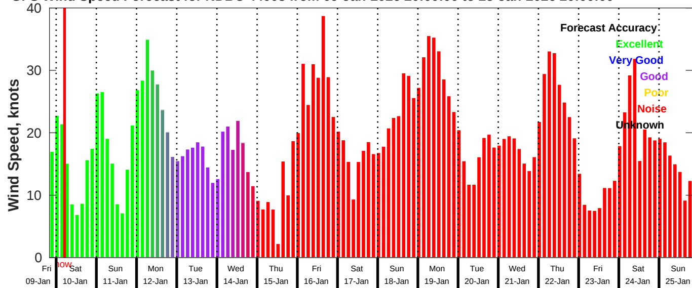
GFS Wind Speed Forecast for NDBC 44008 from 09-Jan-2026 20:00:00 to 25-Jan-2026 20:00:00
