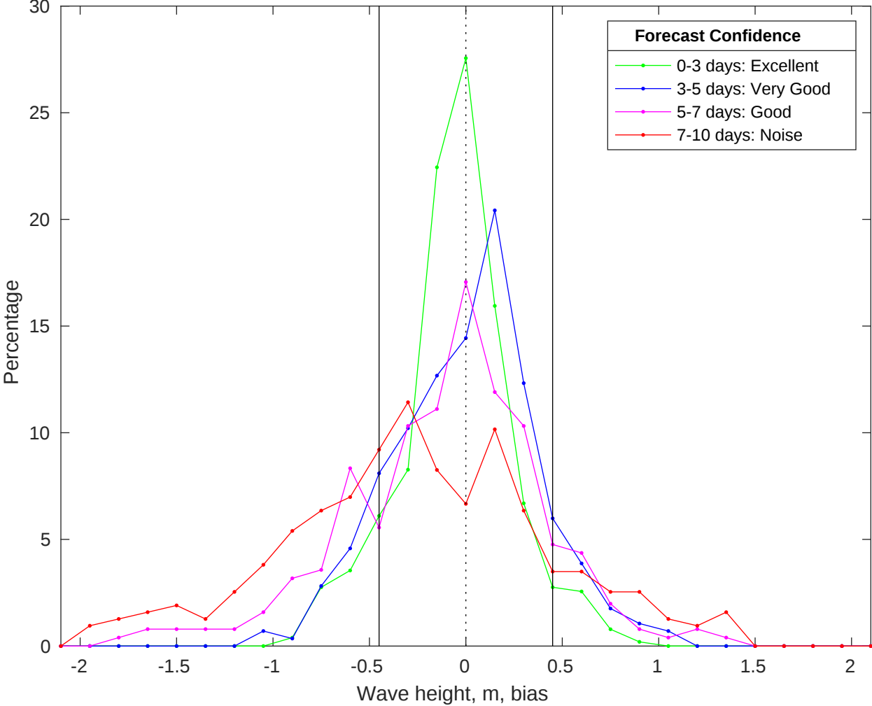
NDBC 46011 vs CMEMS Waves Bias Histogram: 10-Jan-2026
