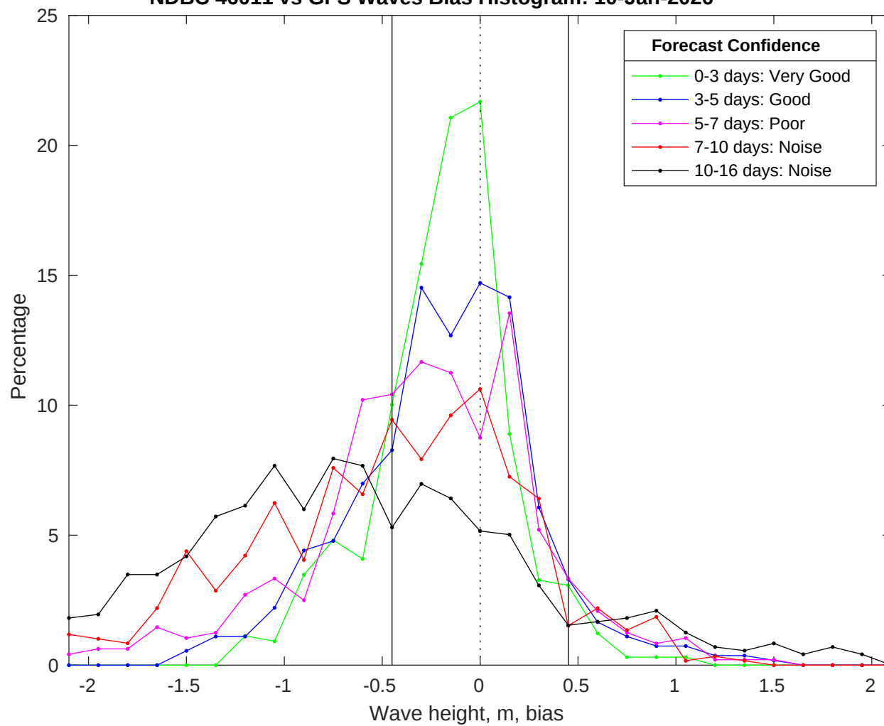
NDBC 46011 vs GFS Waves Bias Histogram: 10-Jan-2026
