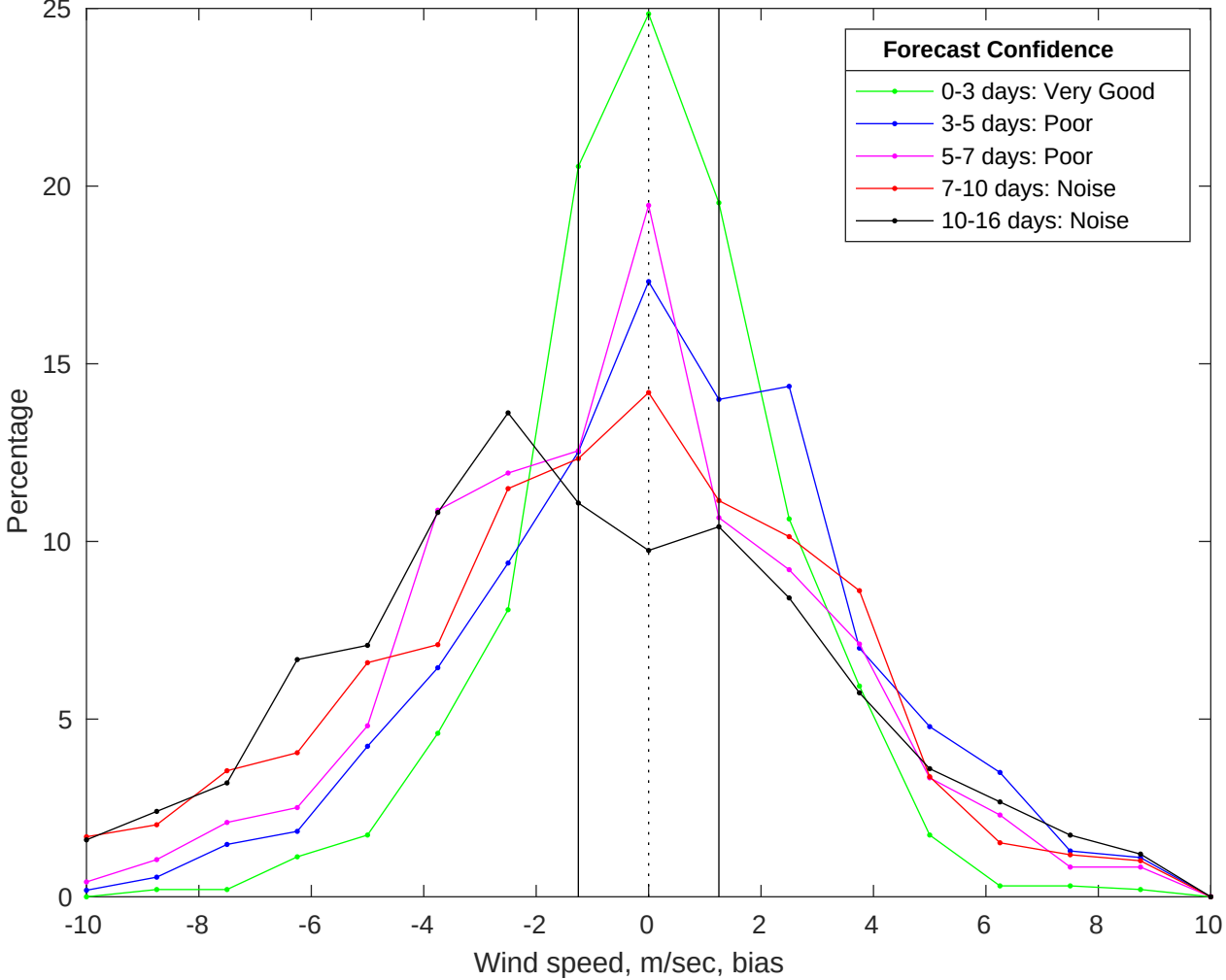
NDBC 46011 vs GFS Winds Bias Histogram: 10-Jan-2026
