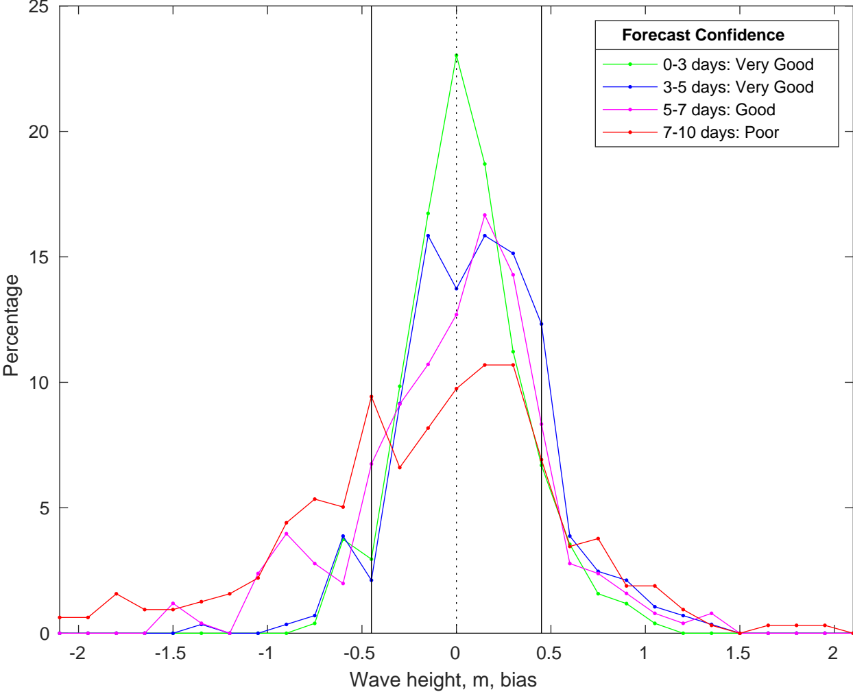
NDBC 46028 vs CMEMS Waves Bias Histogram: 10-Jan-2026
