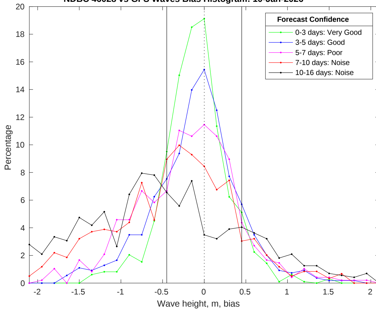
NDBC 46028 vs GFS Waves Bias Histogram: 10-Jan-2026
