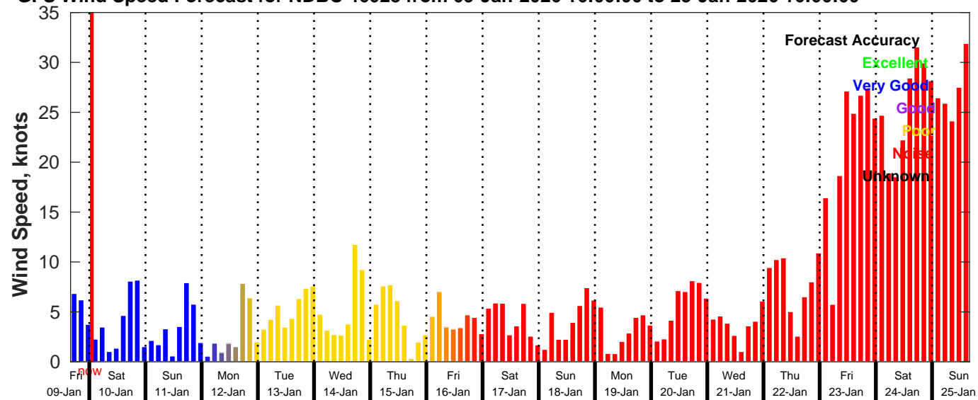
GFS Wind Speed Forecast for NDBC 46028 from 09-Jan-2026 16:00:00 to 25-Jan-2026 16:00:00
