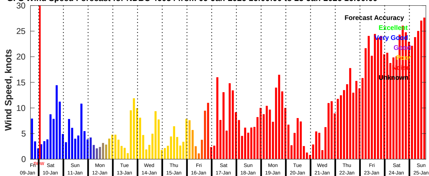
GFS Wind Speed Forecast for NDBC 46054 from 09-Jan-2026 16:00:00 to 25-Jan-2026 16:00:00
